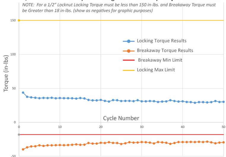
1/2" Locknut — 50-Cycle Locking and Breakaway Torque Trend Results
